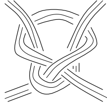
Figure 5. Meshing knot , 10'th knot of Gauss from 1794.
