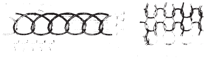
Figure 4. Knots of Vandermonde
