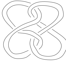
Figure 7. The link of Maxwell.
