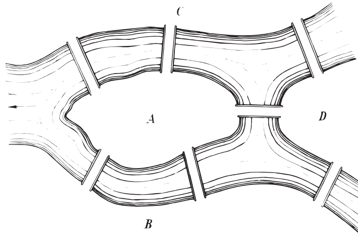
Figure 3. Bridges of Königsberg
