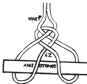
Figure 2. The crossed noose
