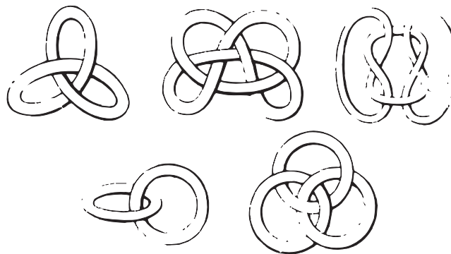
Figure 8. Knots and links of William Thomson (Kelvin) from 1867.
