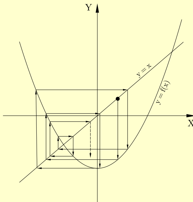
In the above figure f(x) = x^2 - 1.5 .
