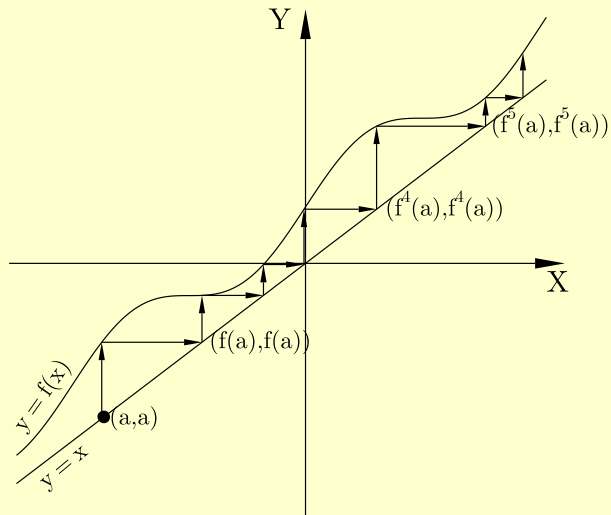
In the above figure f(x) = \sin x + x + 2 .
