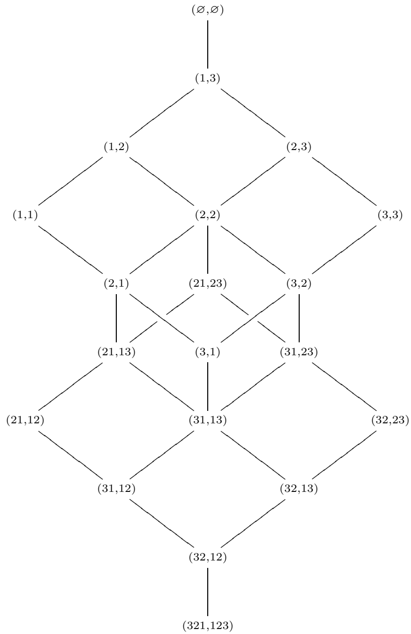
Preferred order of quantum minors
