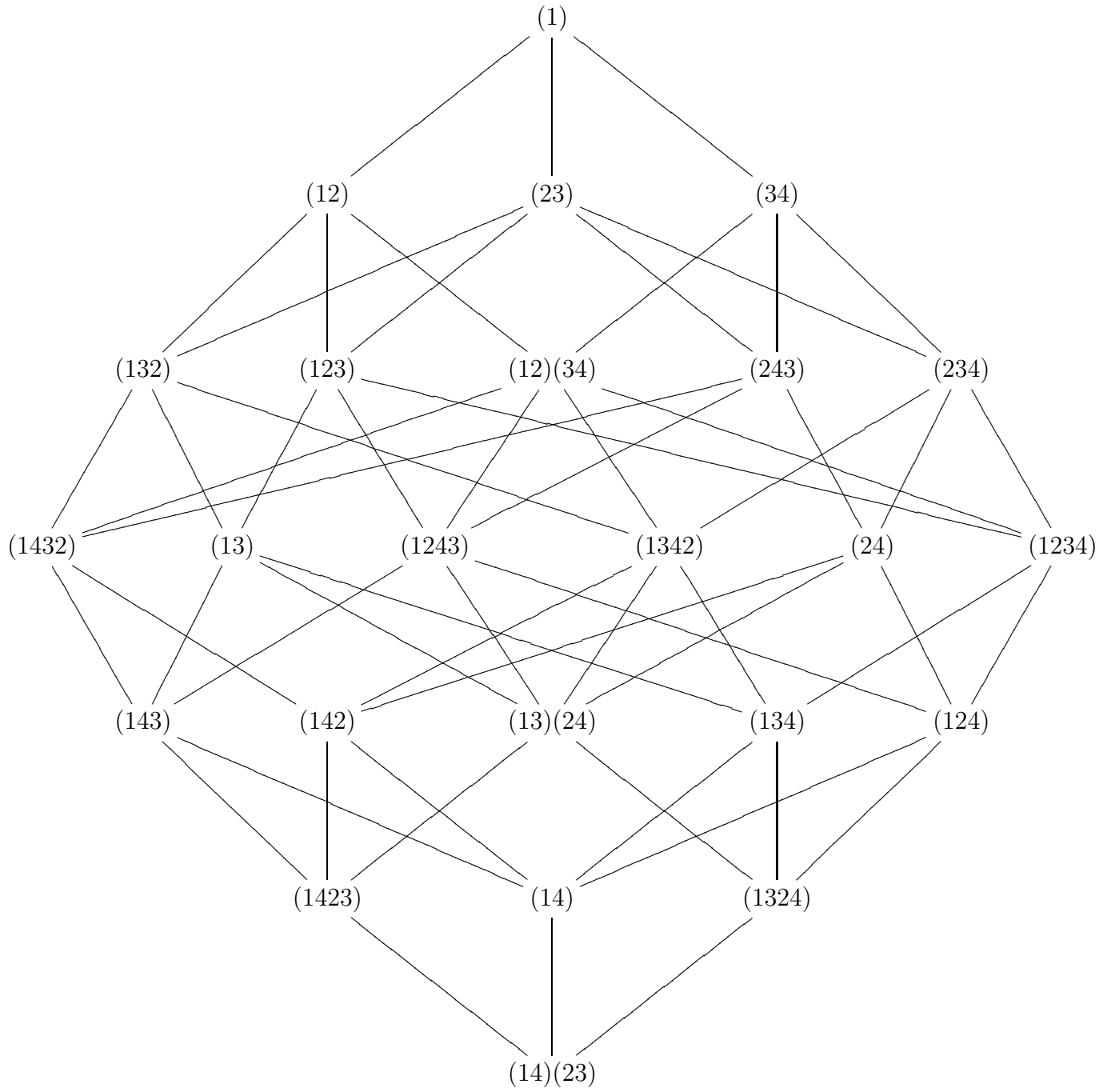
Bruhat ordering of S_4
