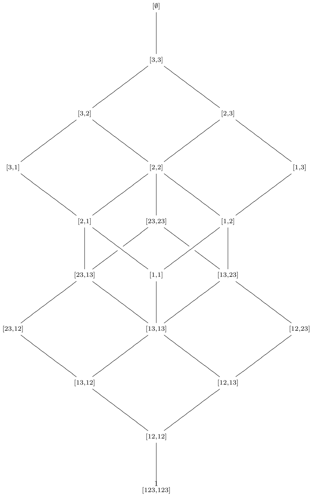
standard order for quantum 3 \times 3 matrices
