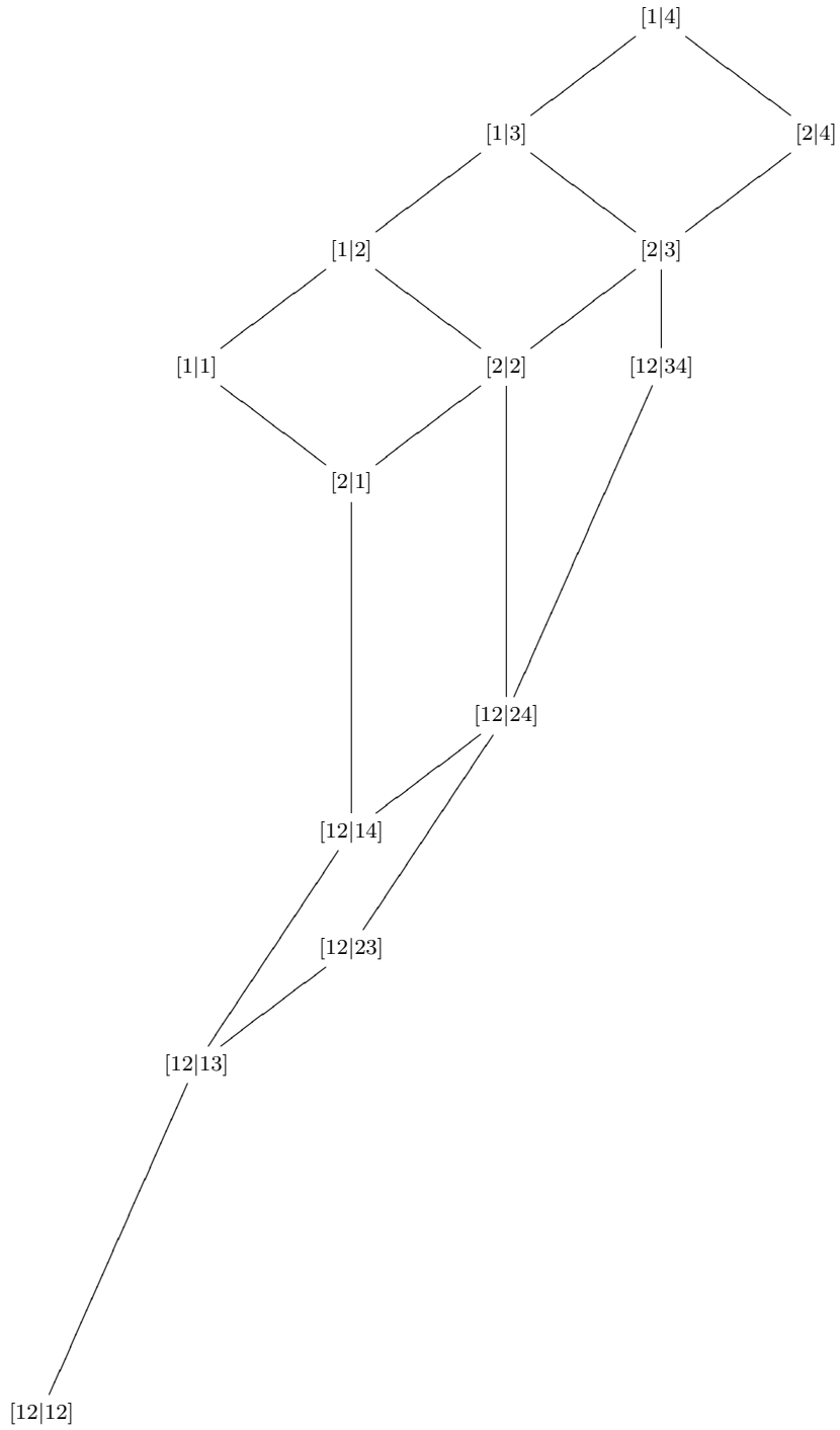
Figure 1: Preferred order of quantum minors in 2 \times 4 quantum matrices
