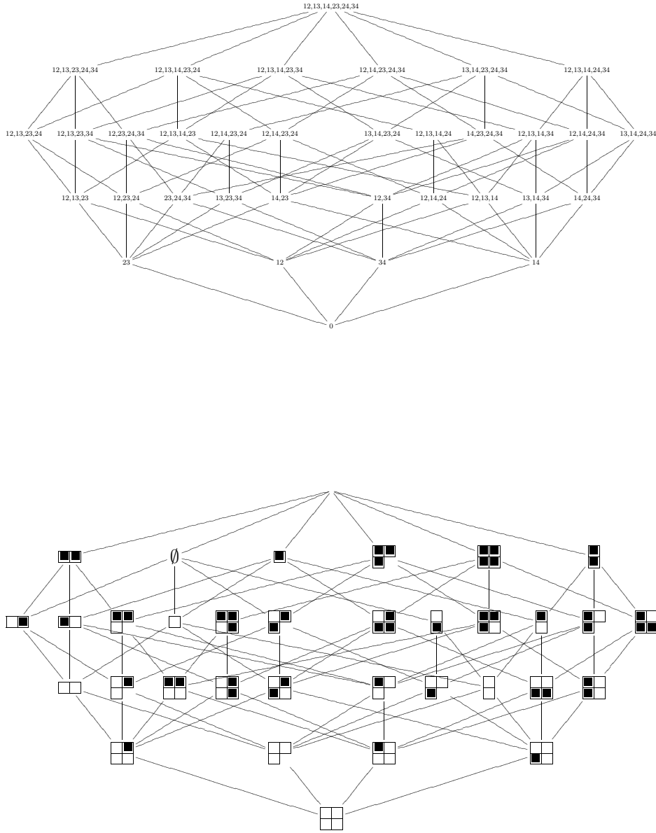
FIGURE 3. The complete \mathcal{H} -prime spectrum of the quantum grassmannian \mathcal{O}_q(G_{2,4}(\mathbb{k})) .
