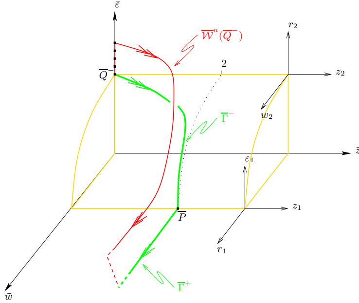
FIGURE 2. The geometry of (11) after blow-up.
