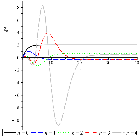
FIGURE 5. The coefficient functions Z_n(w) for n = 0, \dots, 4 and w \in [0, 40] .
