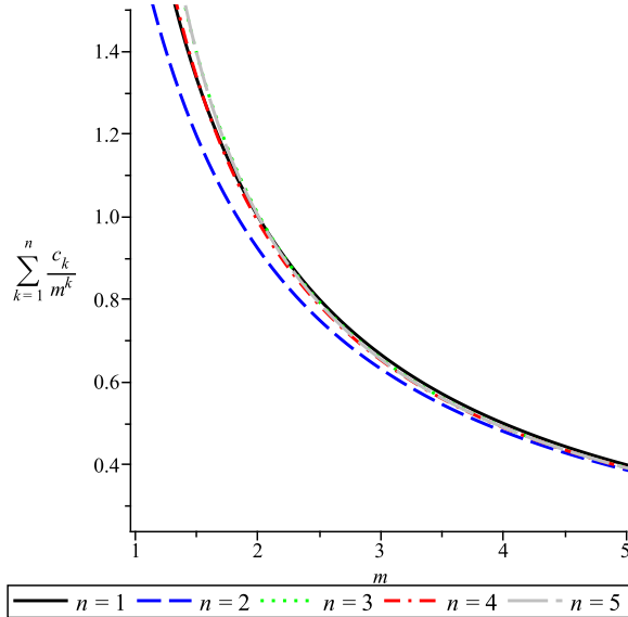
FIGURE 4. The partial sums \sum_{k=1}^n \frac{c_k}{m^k} for n = 1, \dots, 5 and m \in [1, 5] .
