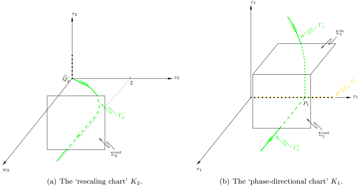
FIGURE 3. The dynamics of the blown-up vector field.
