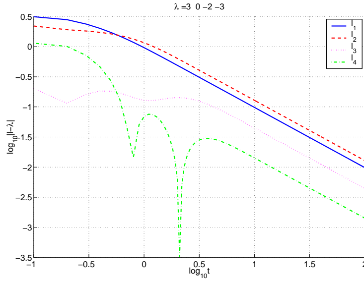
FIG. 4.5. Continuous QR Algorithm , \lambda = \{3, 0, -2, -3\} , PRK4 , \Delta t = 0.1 .
