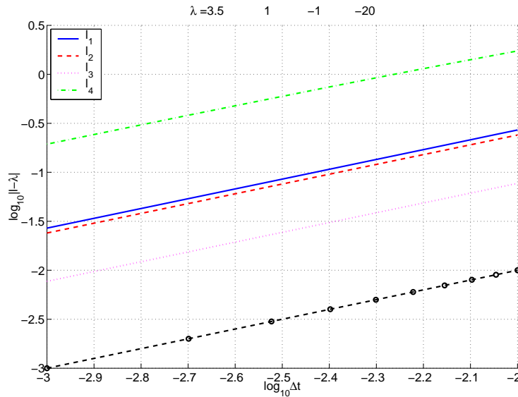
FIG. 4.4. Discrete QR algorithm : \lambda = \{3.5, 1, -1, -20\} , p = 1 , \alpha = 1 .
