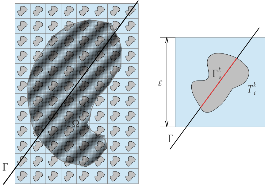
(A) The perforated domain \Omega .
