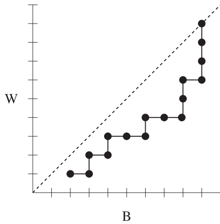
Figure 1. The urn process as a trajectory on a two-dimensional lattice (bold line) where bullets indicate intermediate stages of the trajectory. Exit from the B > W region is equivalent to this trajectory reaching the diagonal (broken line).
