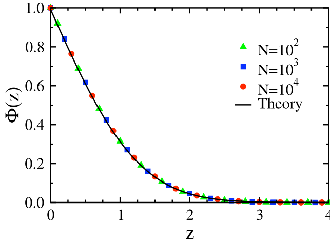
Figure 2. The scaling function \Phi(z) given in (27) versus the scaling variable z (solid line). Also shown is the exit probability E(b, w) , given by the exact expression (13), versus z for three different values of N = b + w (symbols).
