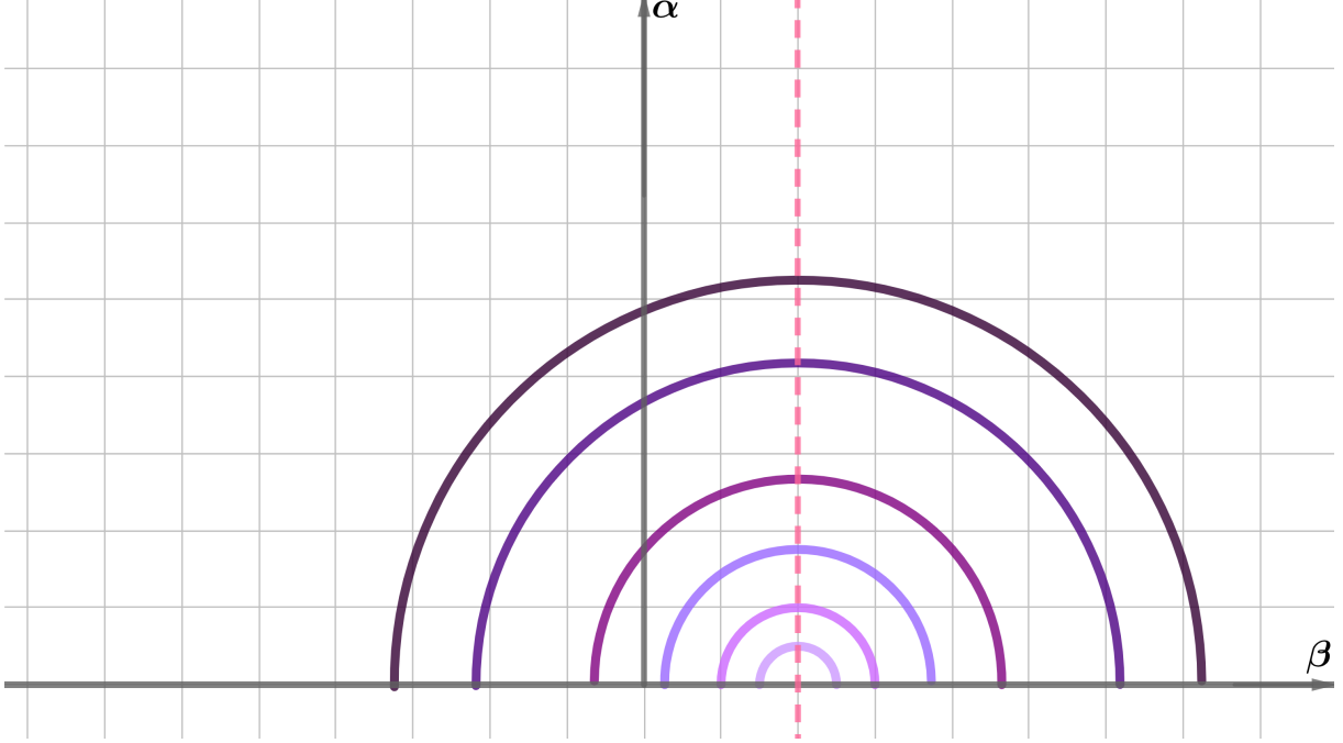
FIGURE 2. Walls are nested semicircles (Theorem 4.12 (iii))
