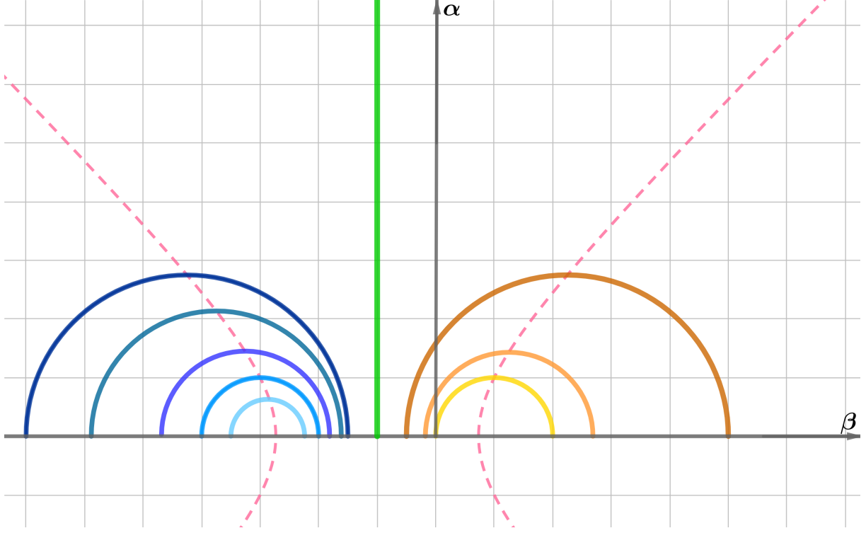
FIGURE 1. Walls are nested semicircles or a unique vertical wall (Theorem 4.12 (ii))
