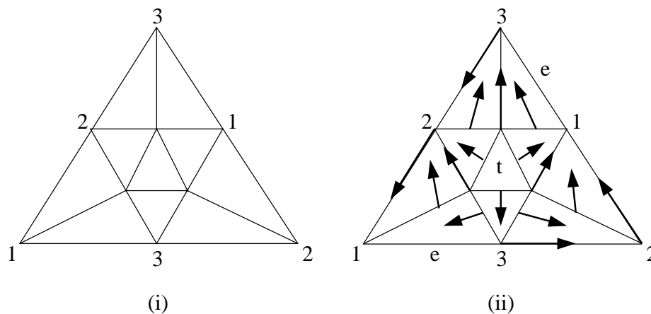
(i) A triangulation of the real projective plane. (ii) A discrete gradient vector field on \mathbb{P}^2 .
