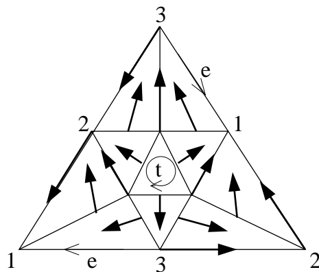
A gradient vector field on the real projective plane.
