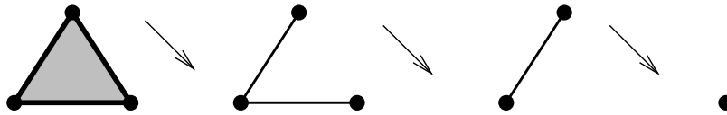
A 2-simplex collapsing to a vertex.
