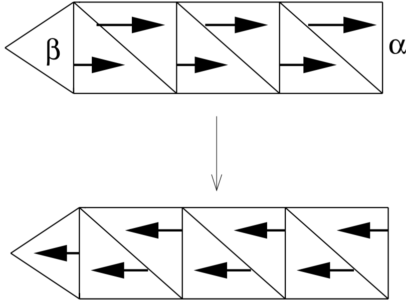
Cancelling critical points.
