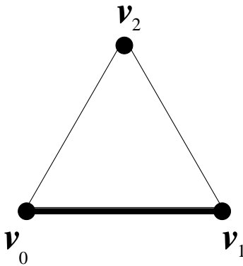
An example of an evasive subcomplex of the 2-dimensional simplex.
