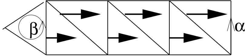
A gradient path from the boundary of \beta to \alpha .
