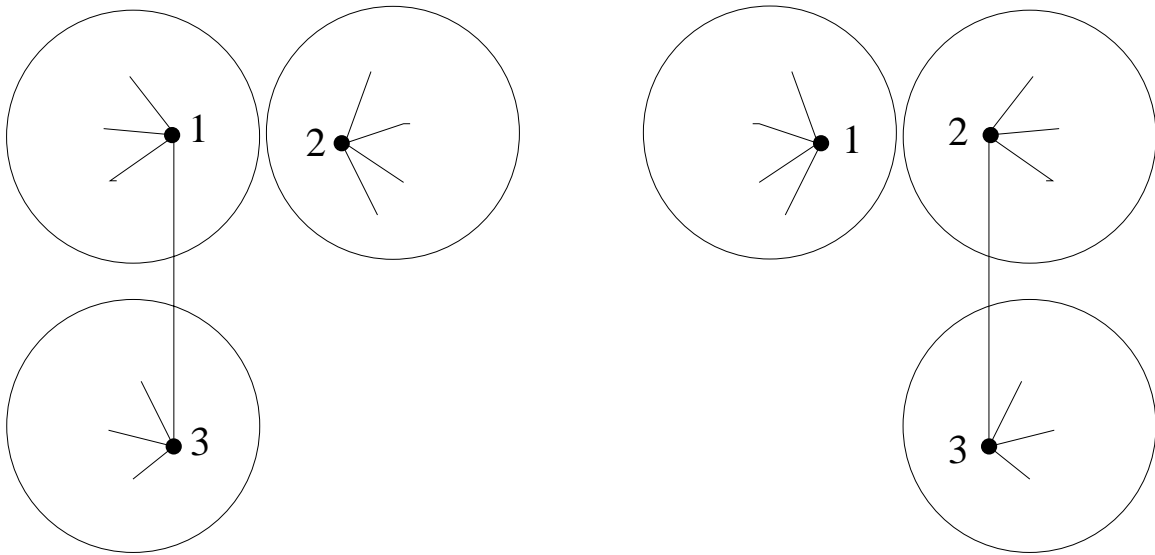
The graphs other than G^* which are unpaired in the vector field V_3 .
