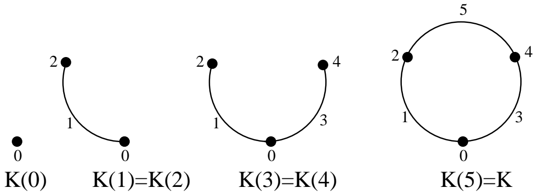
The level subcomplexes of the discrete Morse function shown in Figure 2.2(ii)
