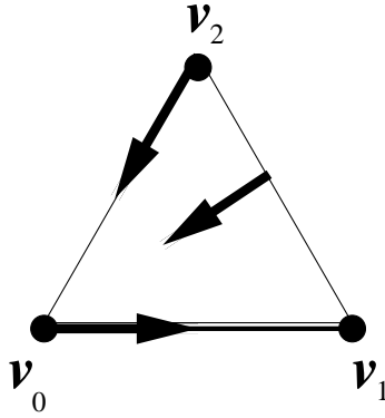
The vector field induced by the guessing algorithm shown in Figure 10.3.
