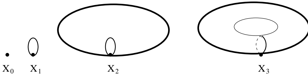
A CW decomposition of a 2-torus
