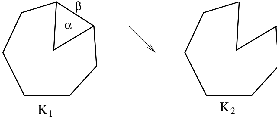
A simplicial collapse.
