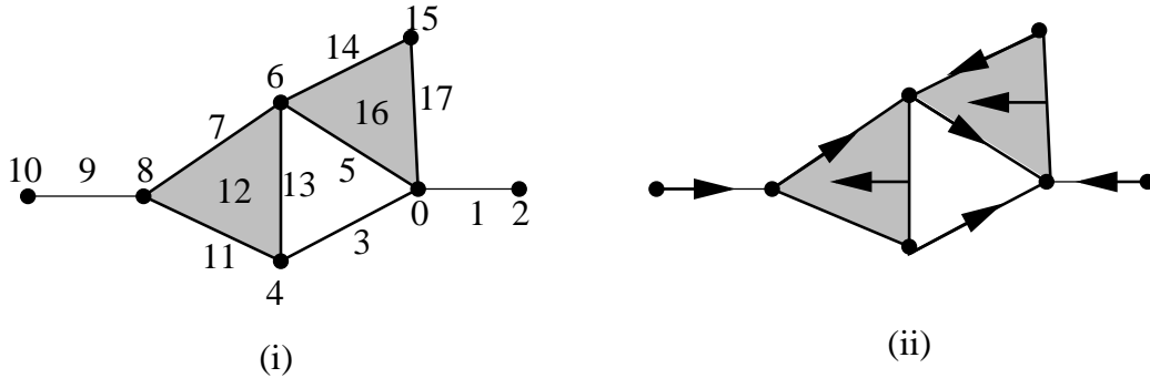
Another example of a gradient vector field
