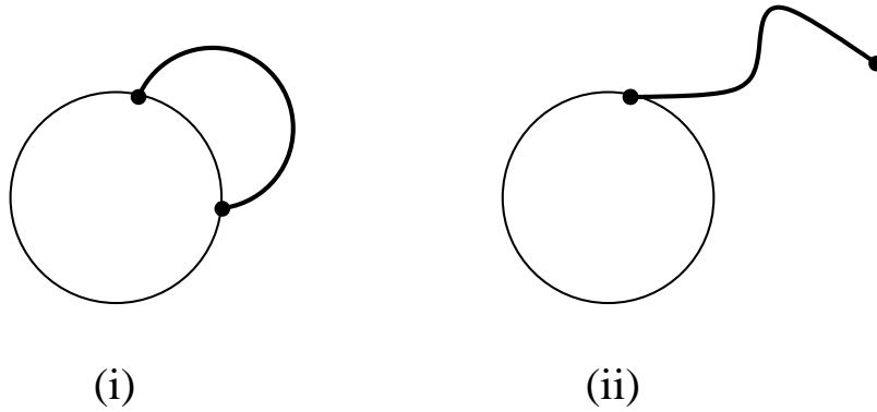
(i). A 1-cell attached to a circle. (ii). This is not a 1-cell attached to a circle
