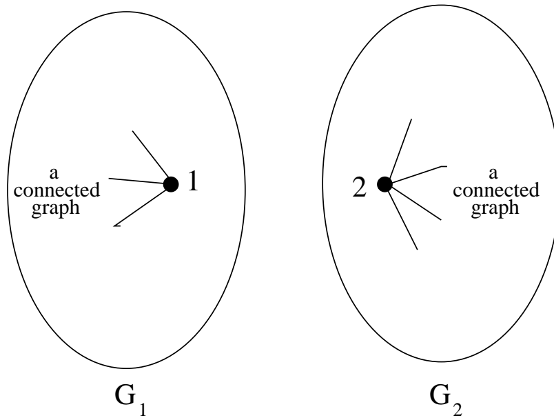
The graphs other than G^* which are unpaired in the vector field V_{12} .
