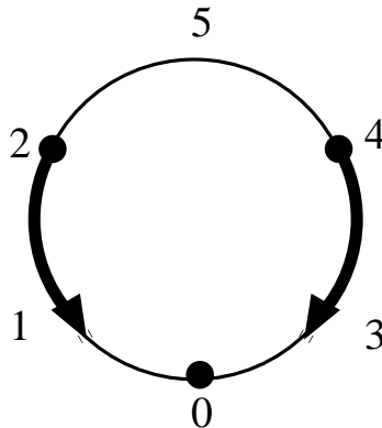
The gradient vector field of the Morse function shown in Figure 2.2 (ii).
