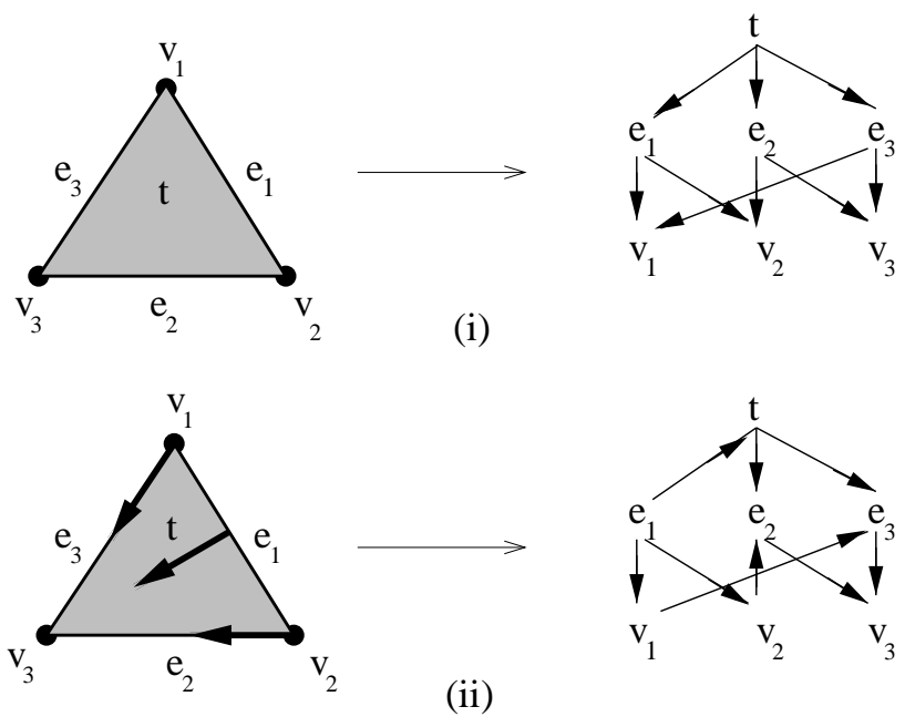
From a discrete vector field to a directed Hasse diagram.
