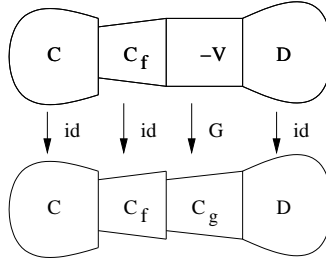
FIGURE 3. The map p_1^*: X_1 \rightarrow X'_1 .
