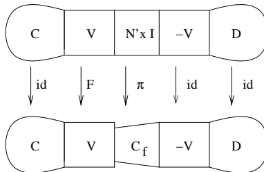
FIGURE 4. The map \phi: M \rightarrow X_1 .
