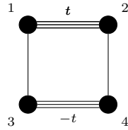
Figure 4.3: The 4-vertex sporadic maximal connected cyclotomic \mathcal{L} -graph \mathcal{S}'_4 . (Where t = 1 + \sqrt{-2} , \frac{3}{2} + \frac{\sqrt{-3}}{2} , \frac{1}{2} + \frac{\sqrt{-11}}{2} for d = -2, -3, -11 respectively.)
