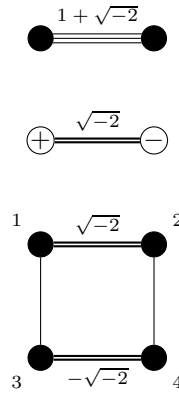
Figure 7.3: The 3-cyclotomic \mathcal{L} -graphs for d = -2 .
