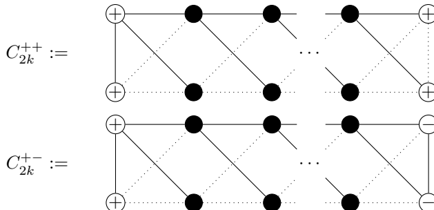
Figure 1.5: The families of 2k -vertex maximal connected cyclotomic cylindrical tessellations C_{2k}^{++} and C_{2k}^{+-} , for k \geq 2 .
