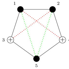
Figure 4.6: The 5-vertex sporadic maximal connected cyclotomic charged \mathcal{L} -graph S_5 .
