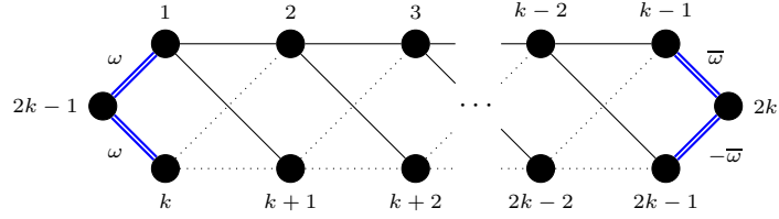
Figure 2.5: The family T_{2k}^{A'} of 2k -vertex maximal connected cyclotomic \mathcal{L} -graphs. (Where k \geq 3 and \omega = \frac{1}{2} + \frac{\sqrt{-7}}{2} .)
