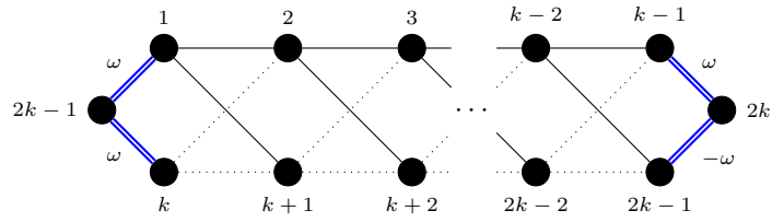
Figure 2.4: The family T_{2k}^A of 2k -vertex maximal connected cyclotomic \mathcal{L} -graphs. (Where k \geq 3 and \omega = 1 + i, \sqrt{-2}, \frac{1}{2} + \frac{\sqrt{-7}}{2} for d = -1, -2, -7 respectively.)
