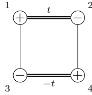
Figure 4.2: The 4-vertex sporadic maximal connected cyclotomic charged \mathcal{L} -graph \mathcal{S}_4 . (Where t = 1 + i , \sqrt{-2} , \frac{1}{2} + \frac{\sqrt{-7}}{2} for d = -1, -2, -7 respectively.)
