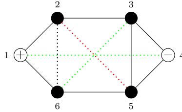
Figure 4.8: The 6-vertex sporadic maximal connected cyclotomic charged \mathcal{L} -graph S'_6 .
