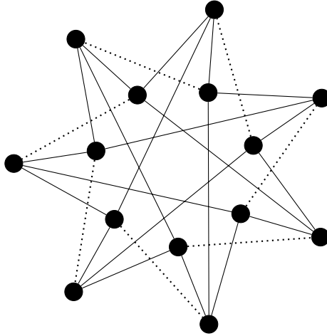
Figure 1.1: The 14-vertex sporadic maximal connected cyclotomic signed graph S_{14} .
