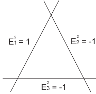
Figure 3.1: Smooth Del Pezzo surface of degree 5
