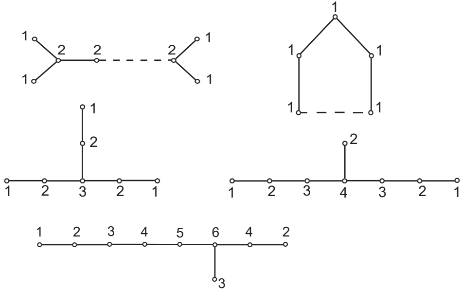
Figure 2.1: Singular fibres
