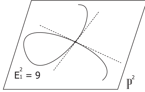
Figure 3.7: Projective plane
