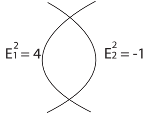
Figure 3.3: Smooth Del Pezzo surface of degree 7
