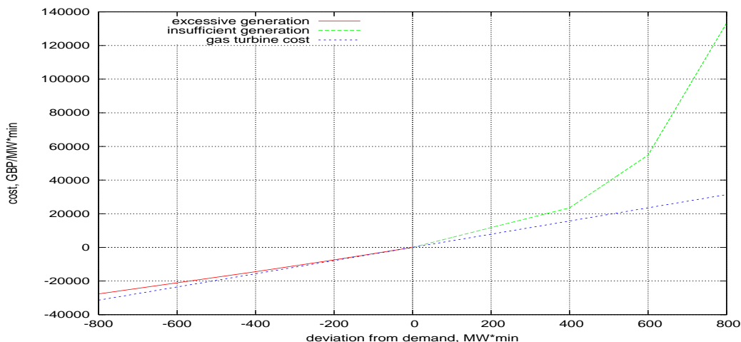
Figure 3.4: Load mismatch costs: the difference between the curves gives the penalty for generation deviating from demand.
