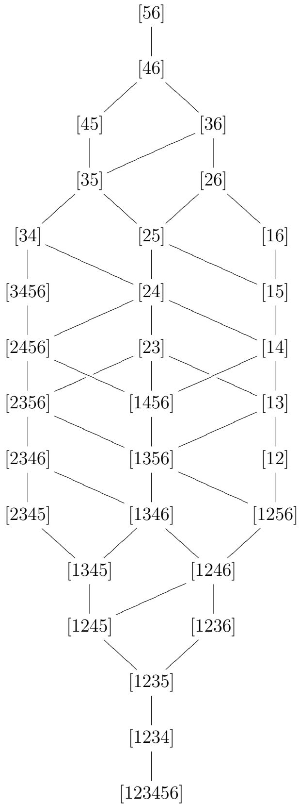
Figure 5.1: The 6 \times 6 Poset
