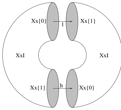
Figure 5.5: Symbolic diagram of CW-mapping torus T(h)
