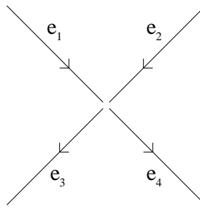
Figure 3.4: A typical crossing in Pk \setminus I
