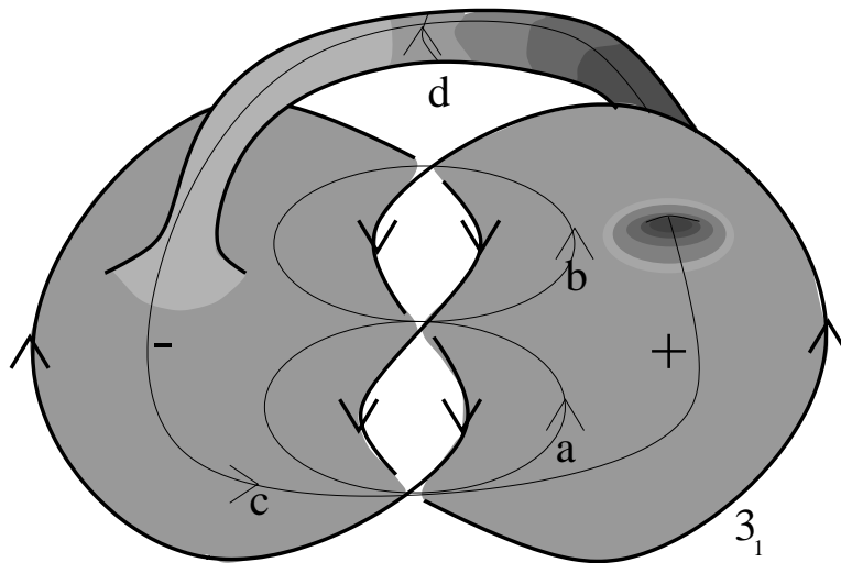
Figure 6.11: Another Seifert surface in the complement of a trefoil knot 3_1
