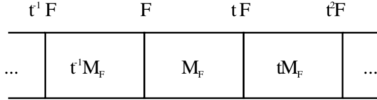
Figure 6.4: Infinite cyclic cover of a knot complement M
