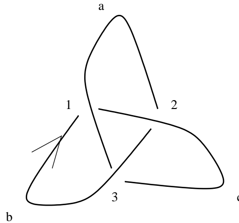
Figure 6.3: A trefoil knot, 3_1 , with labeled arcs and crossings
