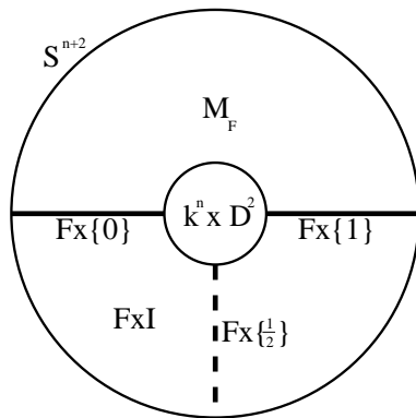
Figure 6.6: A symbolic picture of S^{n+2}
