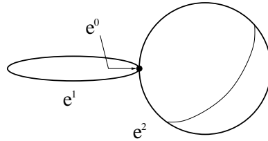
Figure 5.1: V = S^1 \vee S^2
