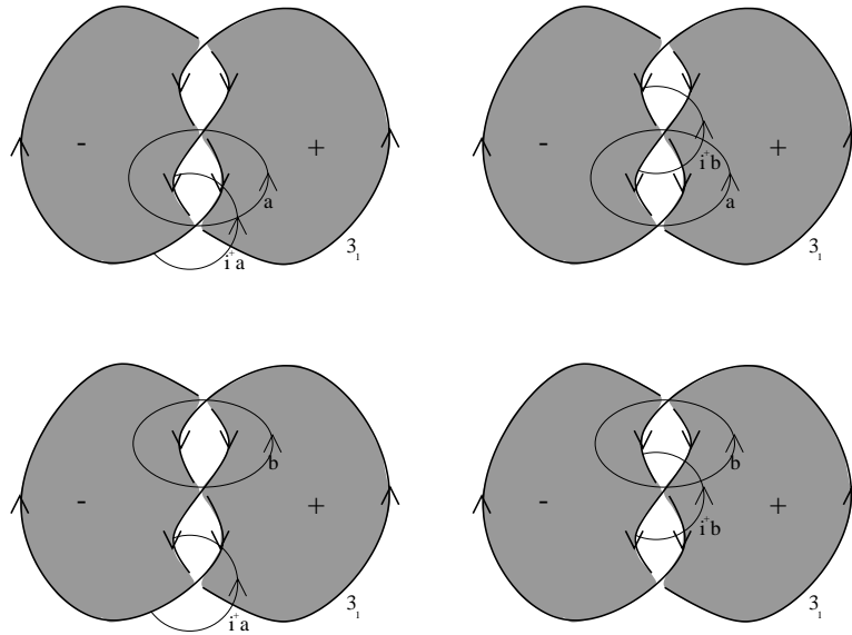
Figure 6.8: Linking the homology generators for H_1(F_{3_1})
