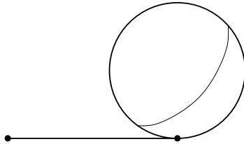
Figure 5.3: A (geometric) fundamental domain of \overline{V} , which is also a subcomplex.
