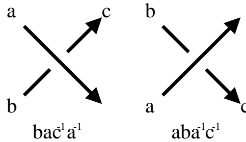
Figure 6.2: Two oriented crossings, and their relations
