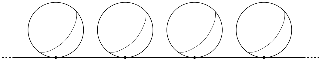
Figure 5.2: \overline{V} = \mathbb{R} \cup_{\mathbb{Z}} (\mathbb{Z} \times S^2)
